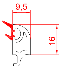
Double Glaze Bead - 9.5 RSB-9.5 DGB
