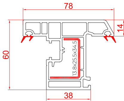
Outward Window Sash - 78 RSC - 78 WO
