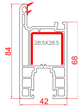
Big Sash - 84 RSS-84BS
