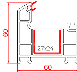
Casement Outer - 60 RSC - 60 OF
