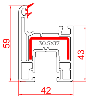
Small Sash - 59 RSS-59SS
