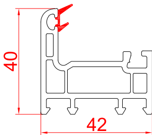
Small Casement Frame - 42 RSC-42EVF
