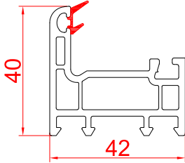
Small Casement Frame - 42 RSC - 42VF
