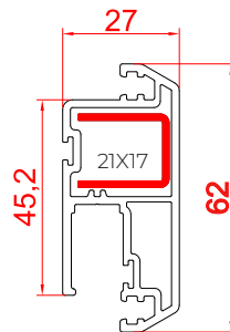
Mesh Mullion - 62 RSM-62MM
