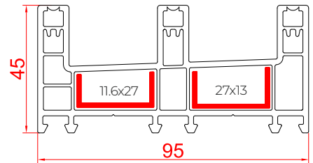
3 Track - 95 Series RST-95ET
