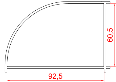
Baypole 60-92 RSA - 92B
