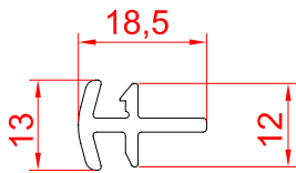
H-Coupler RSA - HC
