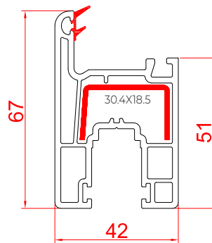
Medium Sash - 67 RSS-67MS
