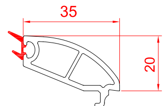
Casement Big Bead - 35 RSB - 35 CB
