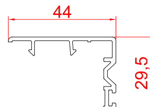
Inter Lock - 44 RSI-44IL
