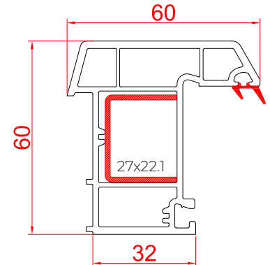
Casement Fly Mullion RSC - 60FM
