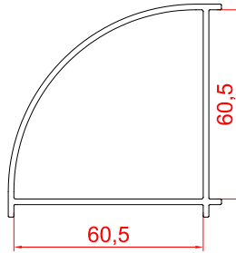
Baypole 60-60 RSA - 60B
