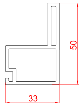
Add On Track RSA - 50 AT
