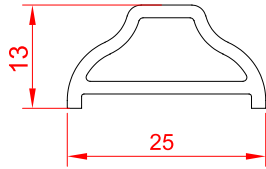
Gorgian Bar RSA - 25 GB
