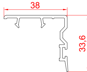
Interlock - Small RSI-38EIL
