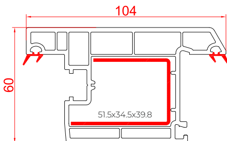
Casement Outward Door Sash RSC - 104 OD
