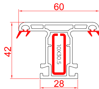
Sash Mullion - 42 RSM-42SM
